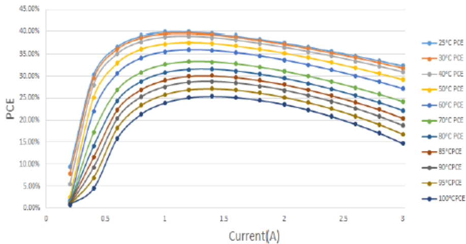
940,2W PCE vs temperature @0.2ms pulse width, 1% duty cycle
