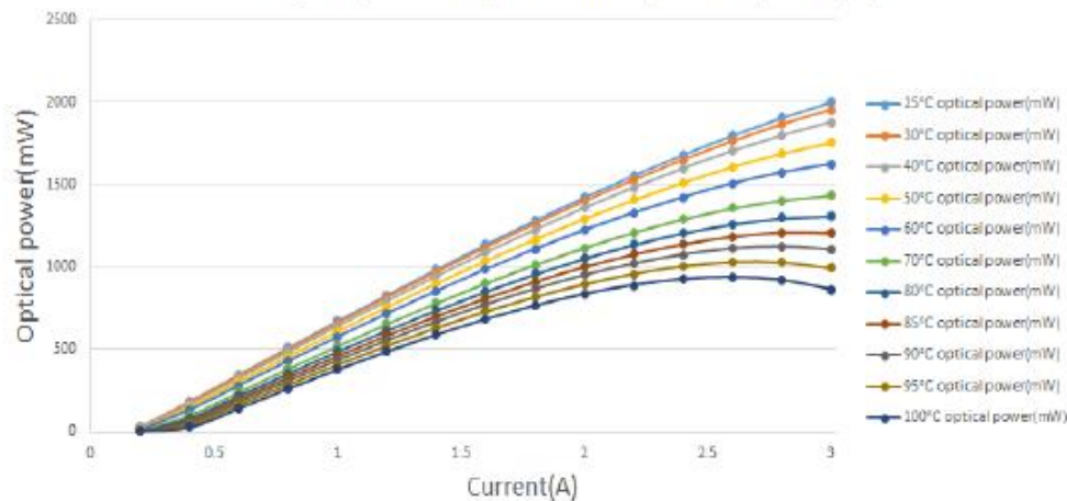
Optical power vs temperature @0.2ms pulse width, 1% duty cycle
