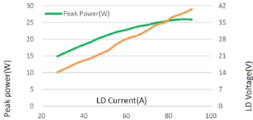
LIV Graph
