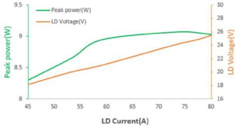
LIV Graph
