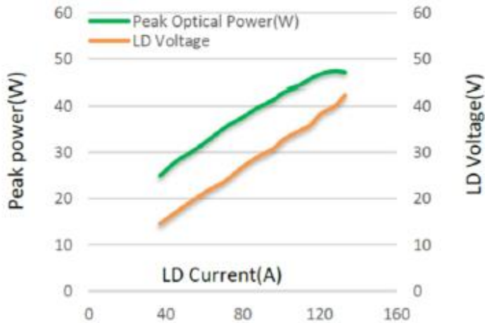
LIV Graph
