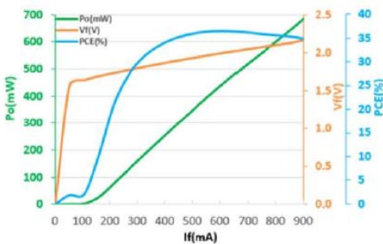
LIV Graph
