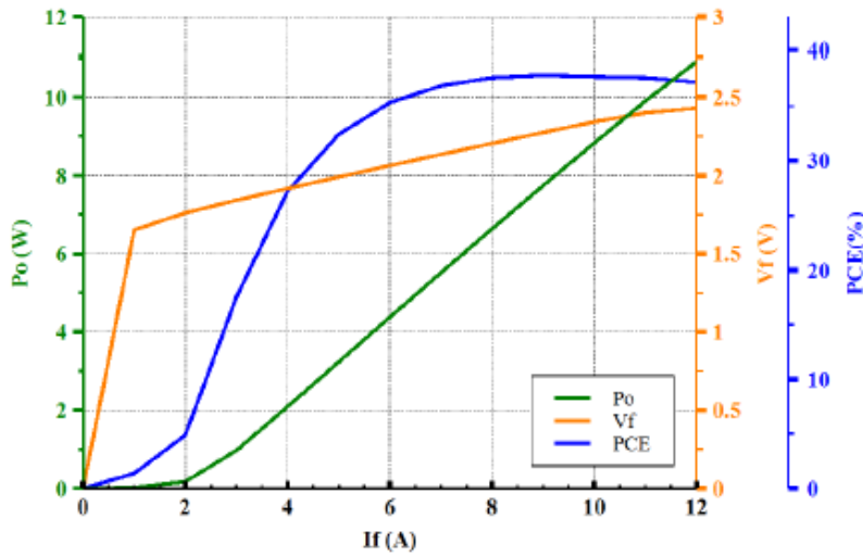
LIV Graph
