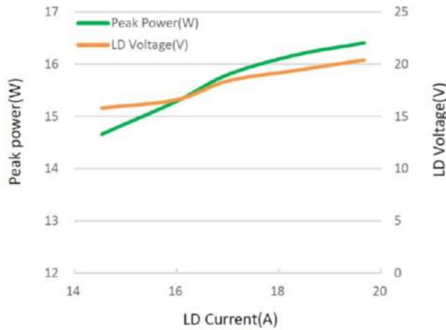
Pulse width=7.2ns
