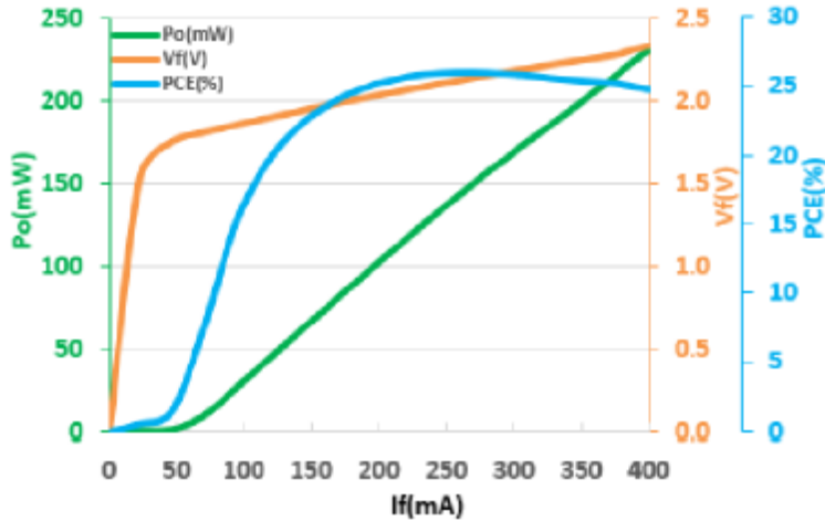
LIV Graph
