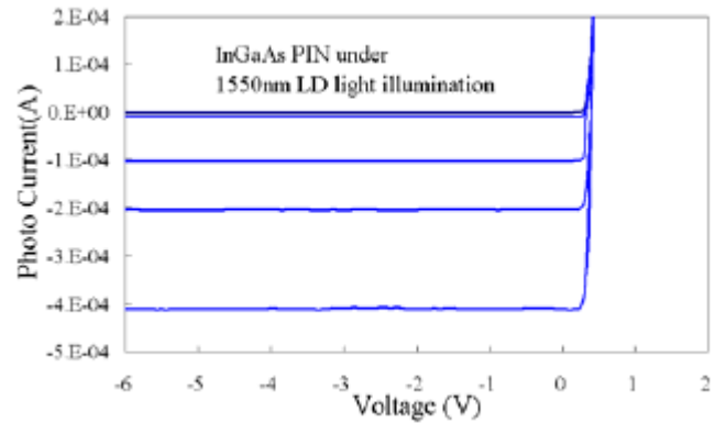
Fig. 2 Typical Photo-Current
