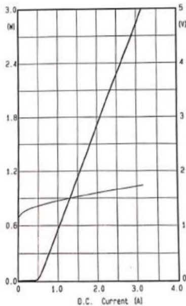
P-I-V Curve
