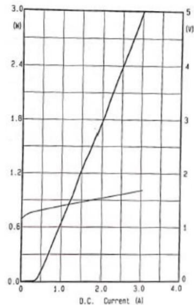
P-I-V Curve
