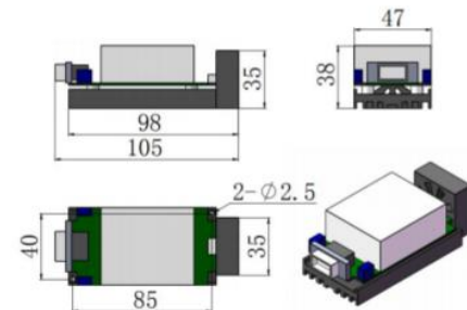
PCB Driver (90-264VAC)
