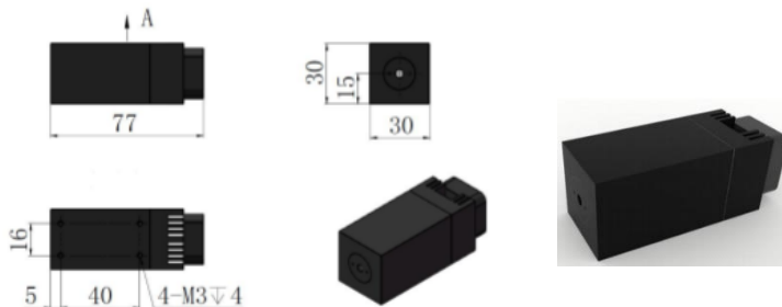
Laser Head
